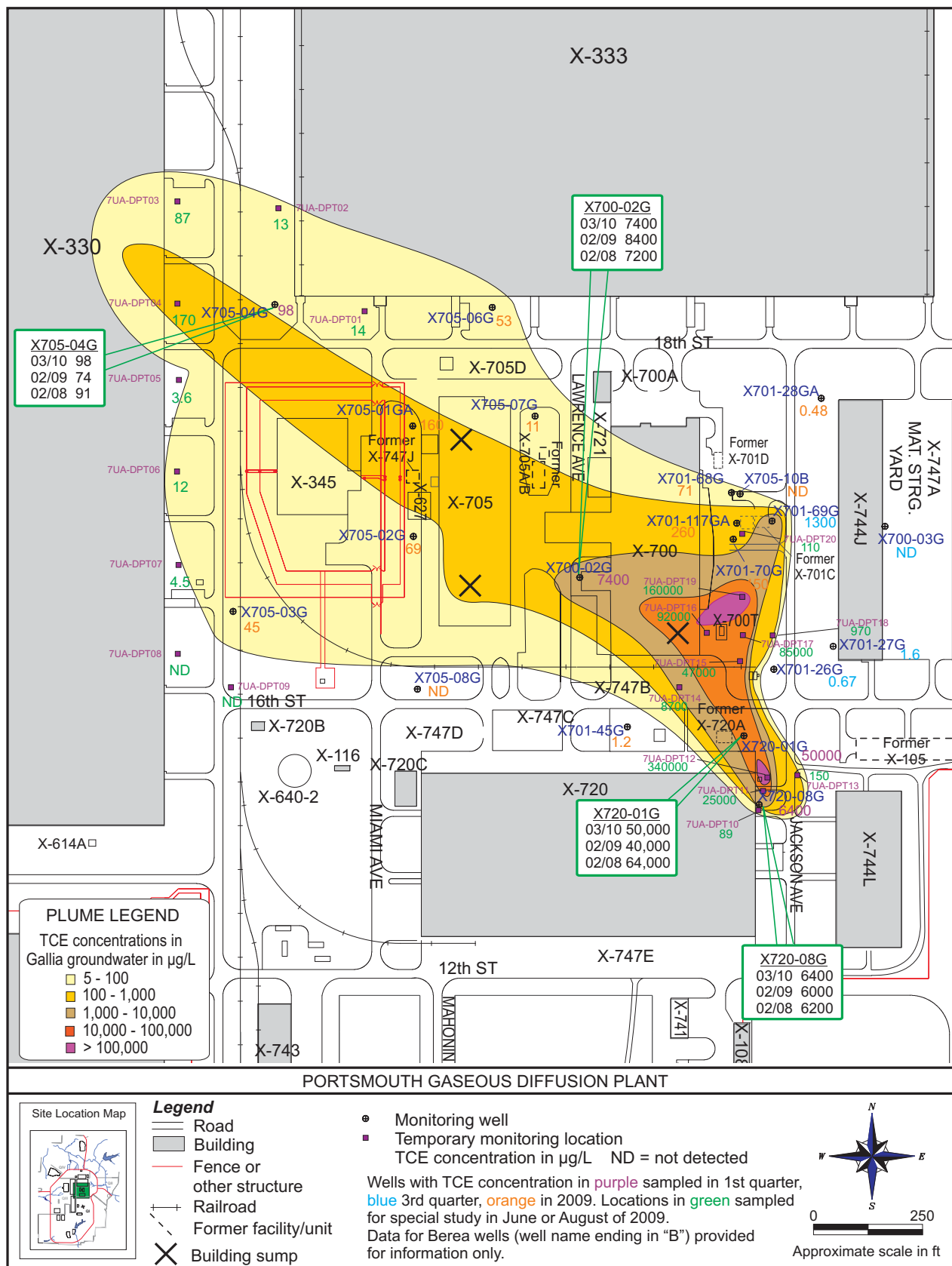
Figure 6.4. Trichloroethene-contaminated Gallia groundwater plume at the Quadrant II Groundwater Investigative Area – 2010.
